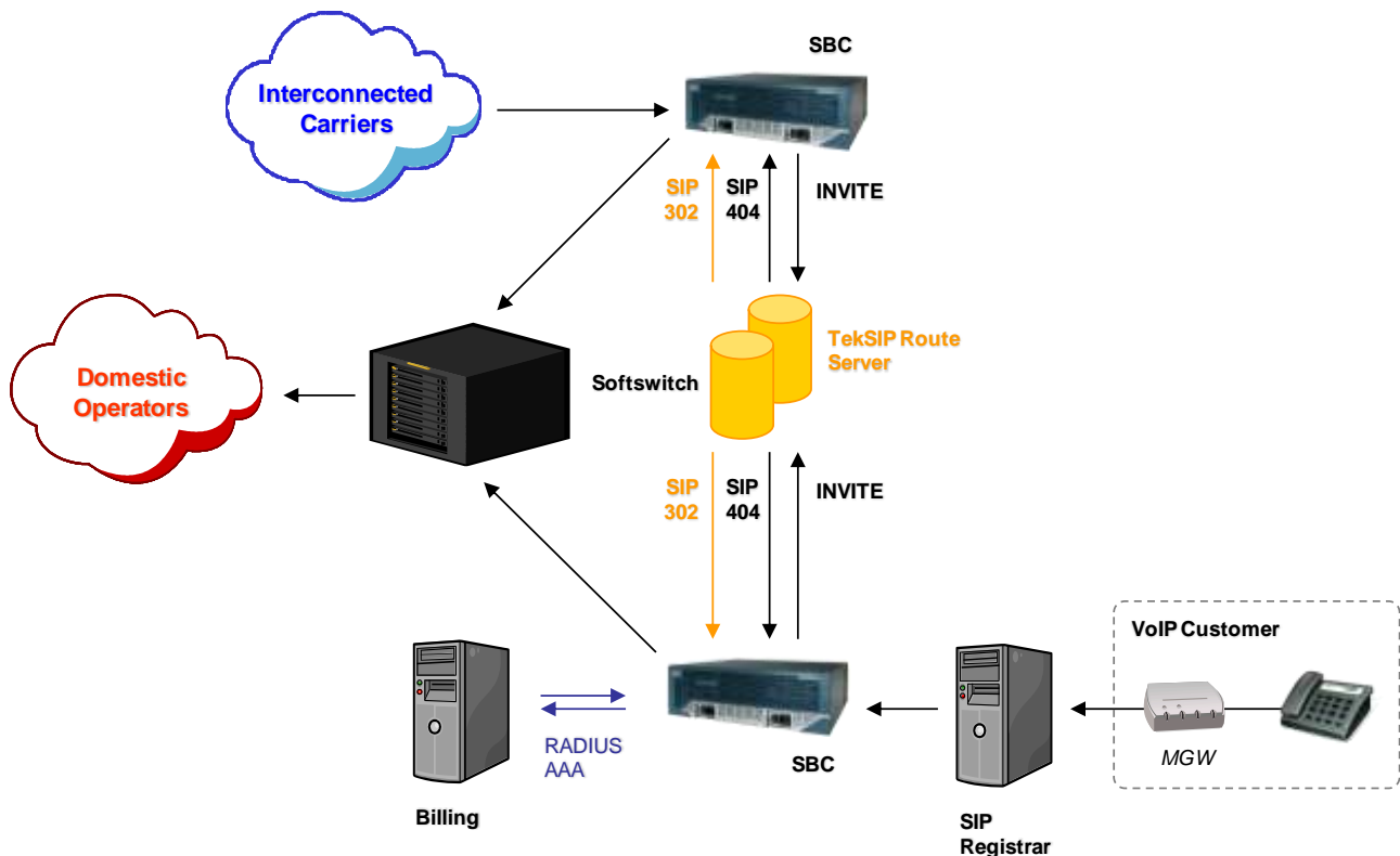
Figure - 4. Number Portability Application Network Diagram
